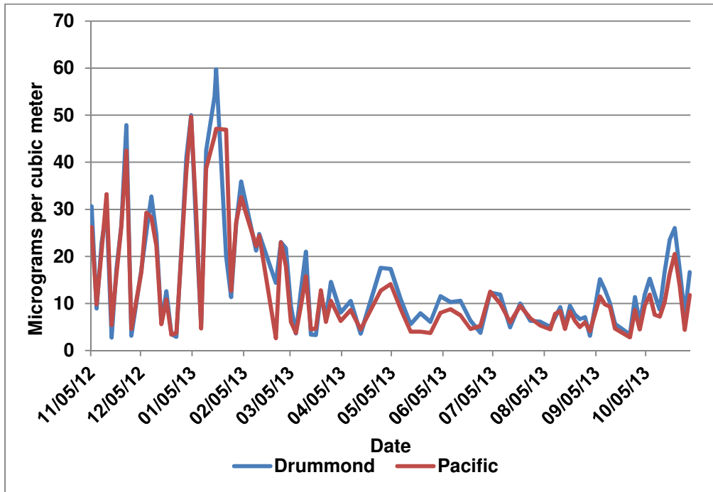
Figure 2: Comparison of PM2.5 Concentrations between Sites during Parallel Monitoring Period (Ascending Fresno-Pacific Values Timeline)
