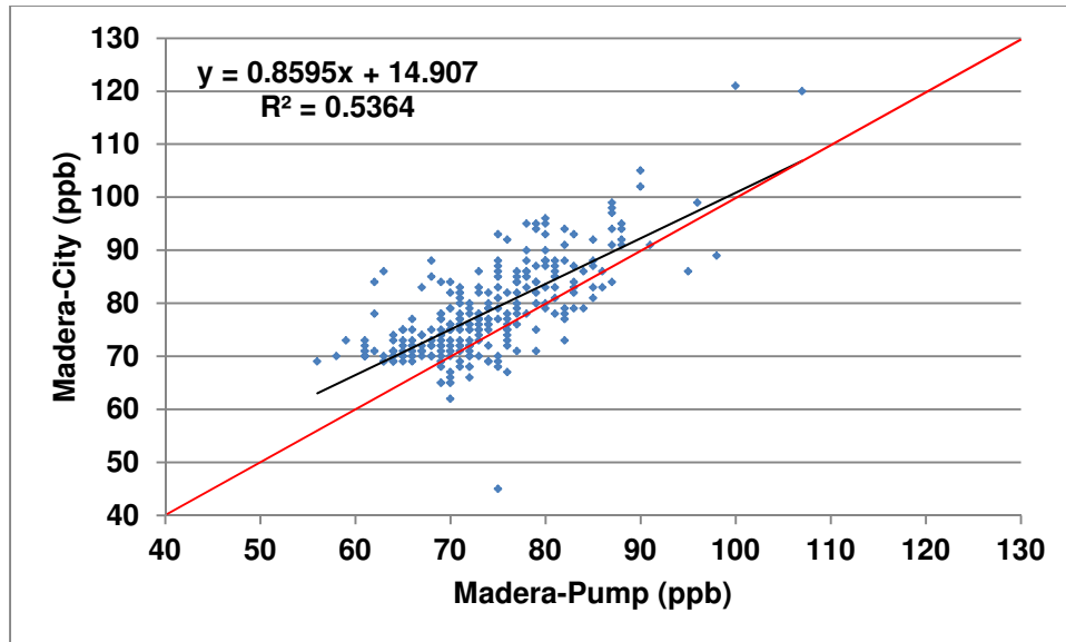
Figure 12: Linear Regression of 8-hour Average Ozone between Madera-Pump and Madera-City Sites
