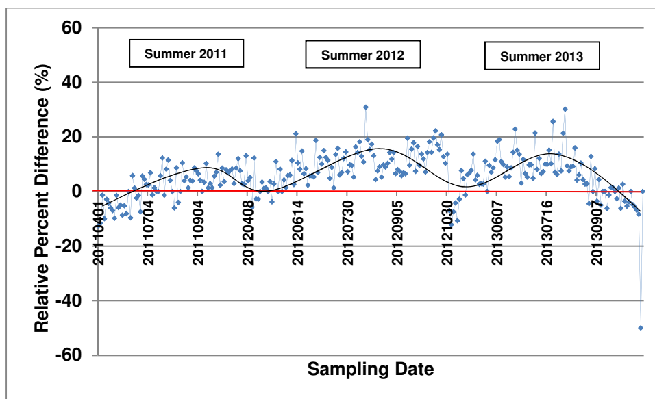
Figure 10: Relative Percent Difference of 8-Hour Average Ozone over Parallel Monitoring Period
