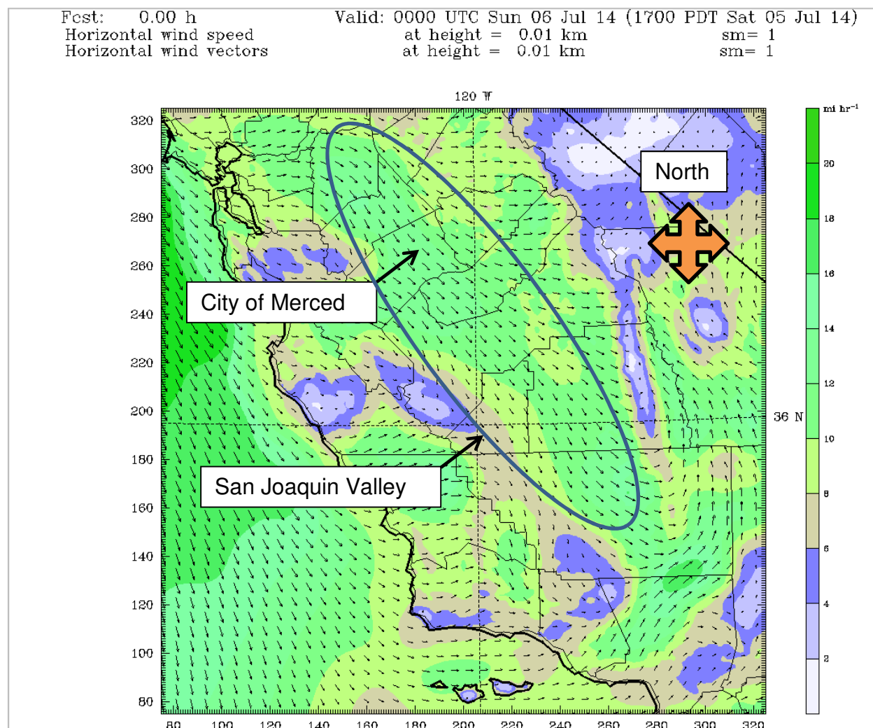
Figure 2: Typical summer wind flow pattern (Arrows depict wind direction, colors depict wind speed)
