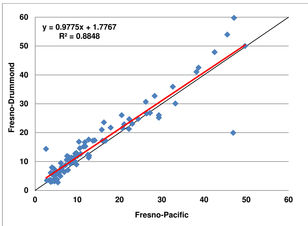
Figure 3: Linear Regression between Fresno-Pacific and Fresno-Drummond PM2.5 Concentrations during Parallel Monitoring Period
