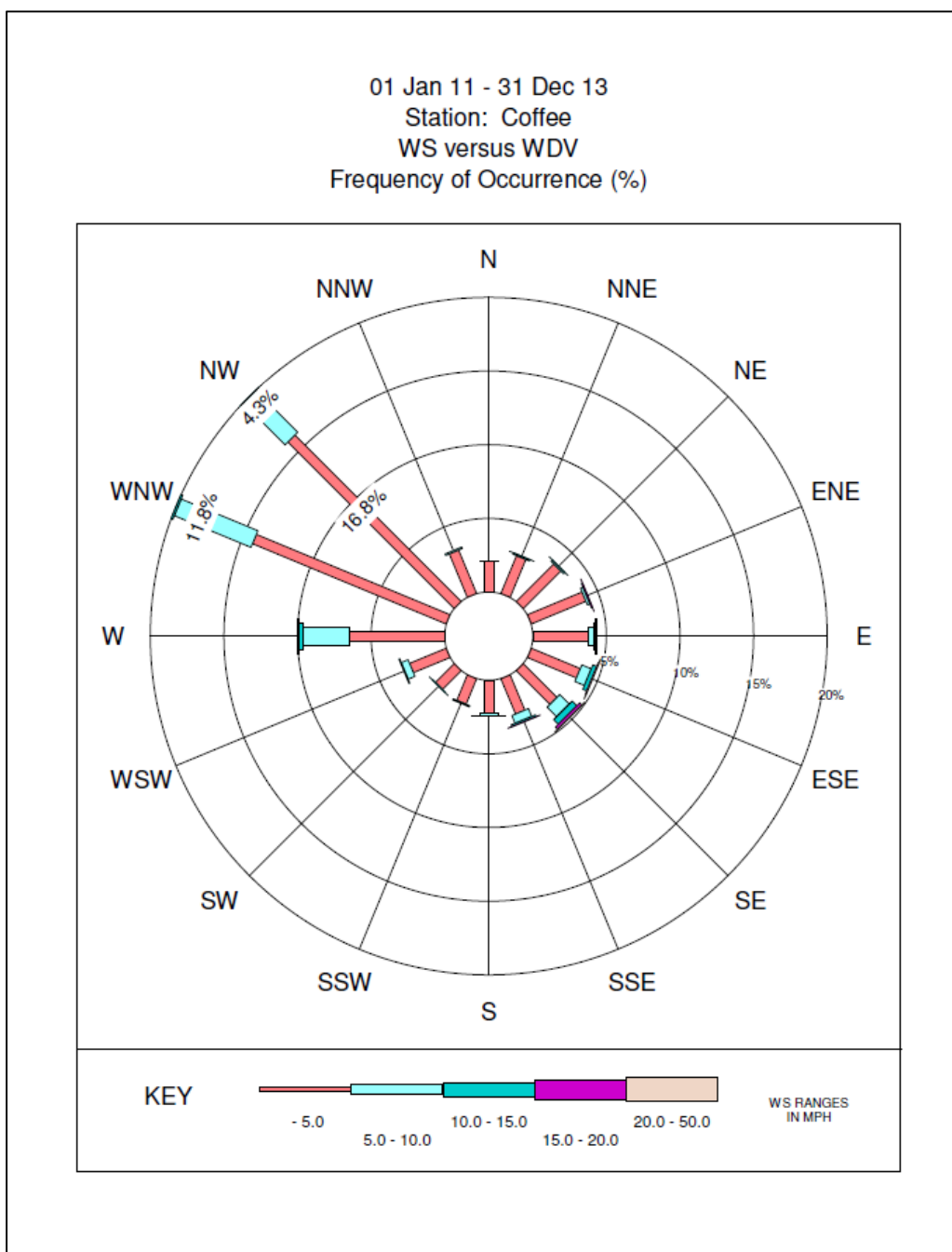
Figure 4: Merced-Coffee Wind Rose for Jan. 1, 2011 through Dec. 31, 2013
