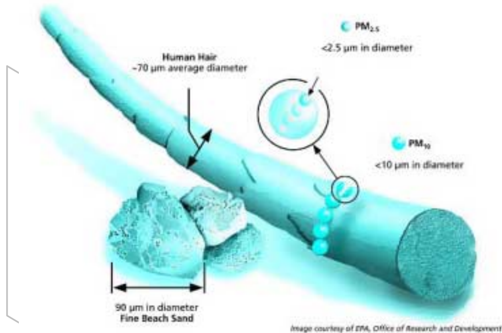
Figure 1-2 Diameter Comparison: Human Hair, Sand, PM10, and PM2.5
