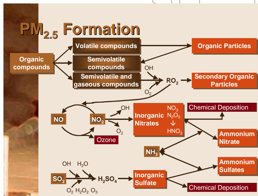
Figure 1-1 PM 2.5 Formation
