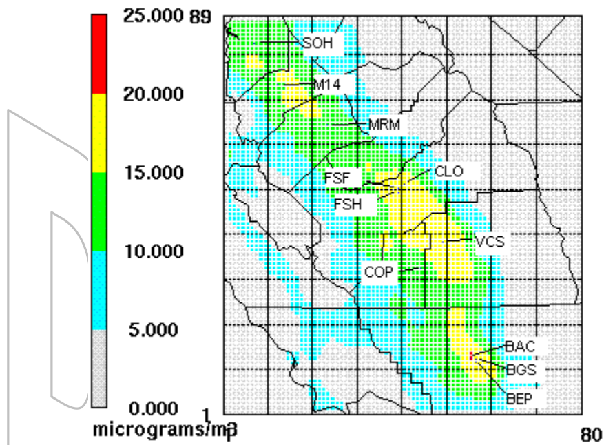
Figure 3. The annual-averaged modeled PM 2.5 concentrations in the domain.
