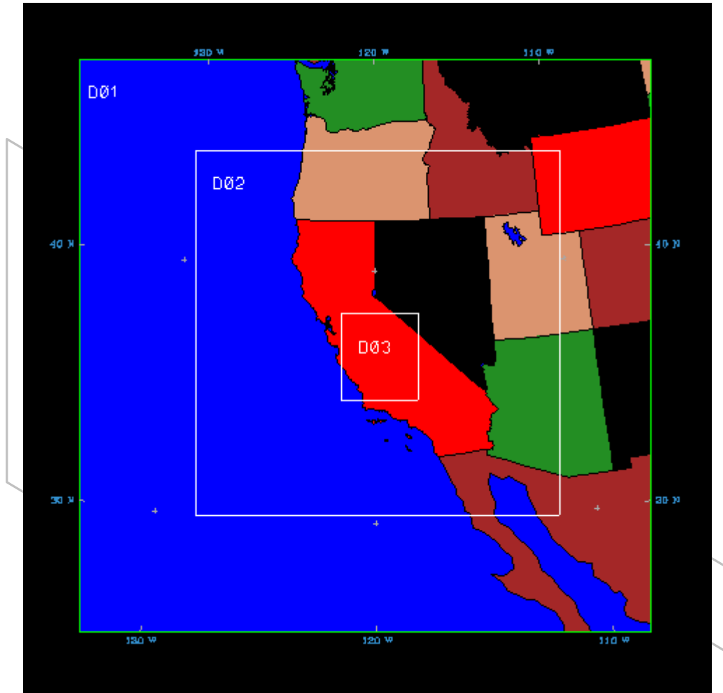
Figure 2. The location of the three nested grids adopted for the numerical modeling of SJV using MM5.
