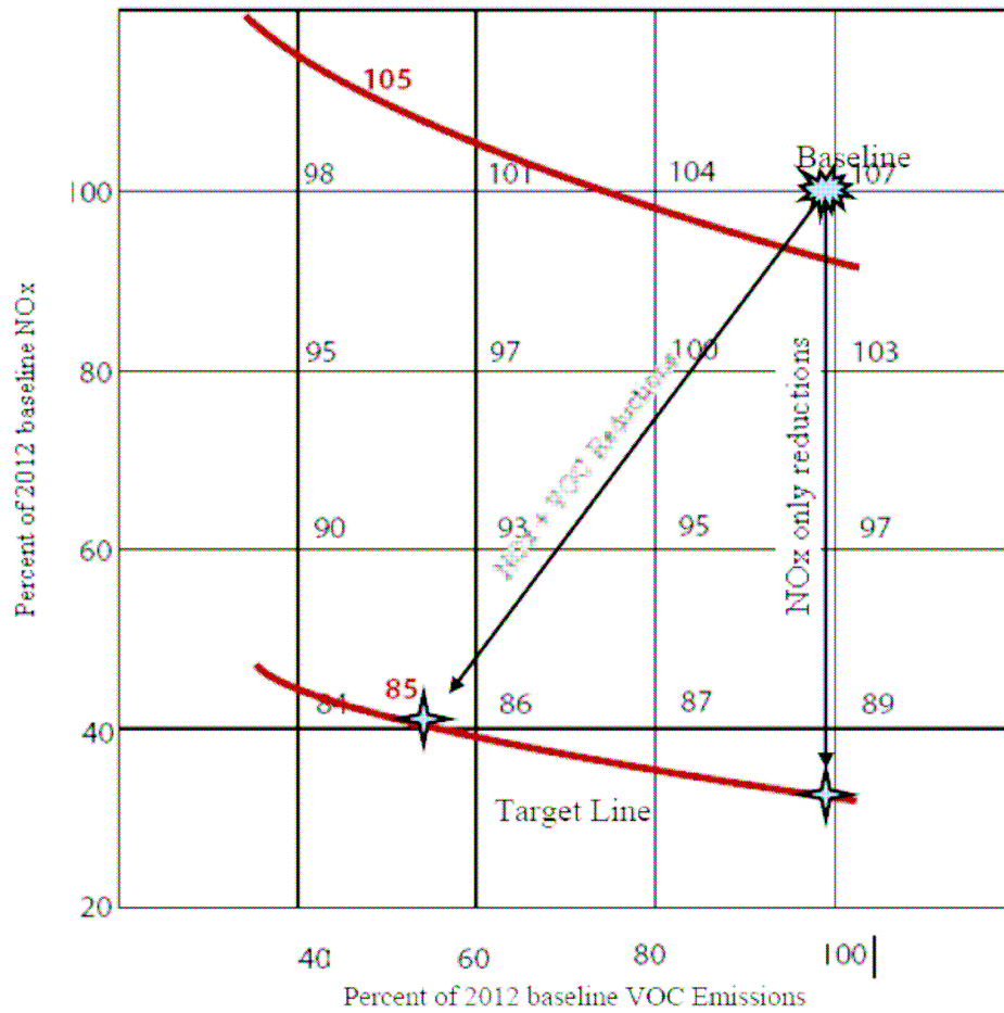
Figure 3-1 Estimation of Carrying Capacity for Arvin
